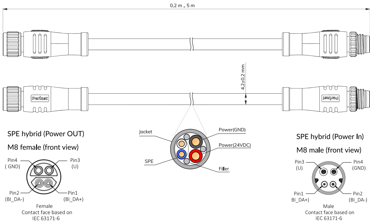
Figure 1: Mechanical Dimensions
